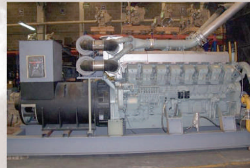
Engine Reconditioned
